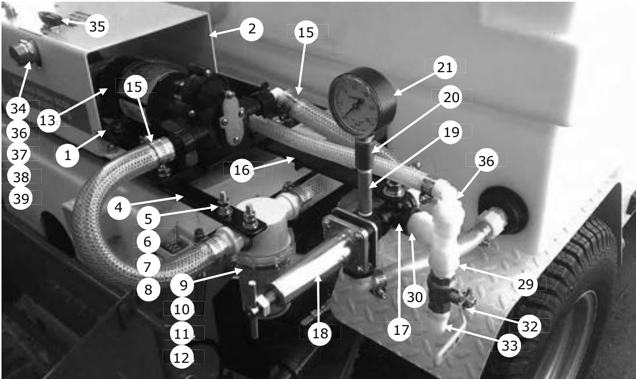
65 Gallon Electric Spray Module (DC65)
