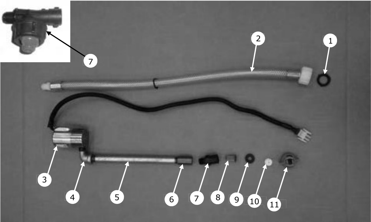
Single Line Painter Dual Color Kit (LP17)
