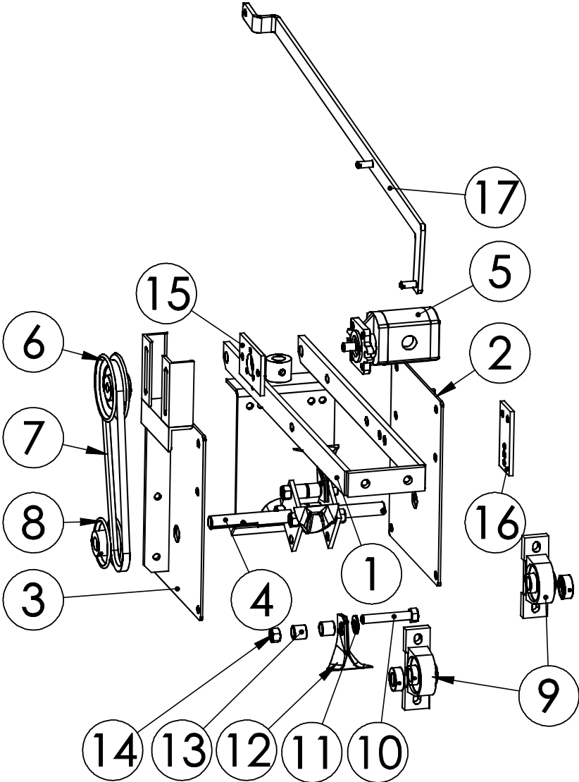
Line Cutter/Painter (LC1) 2 of 2
