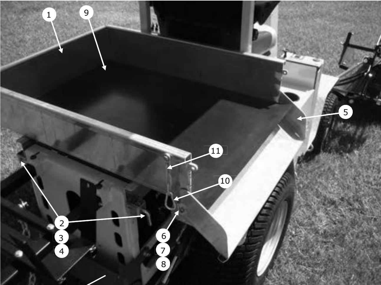
Utility Box (UBS)
