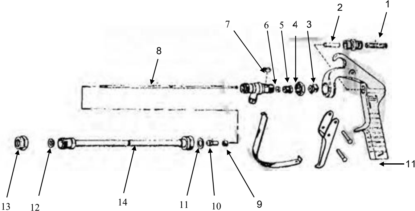
Spray Wand Breakdown
