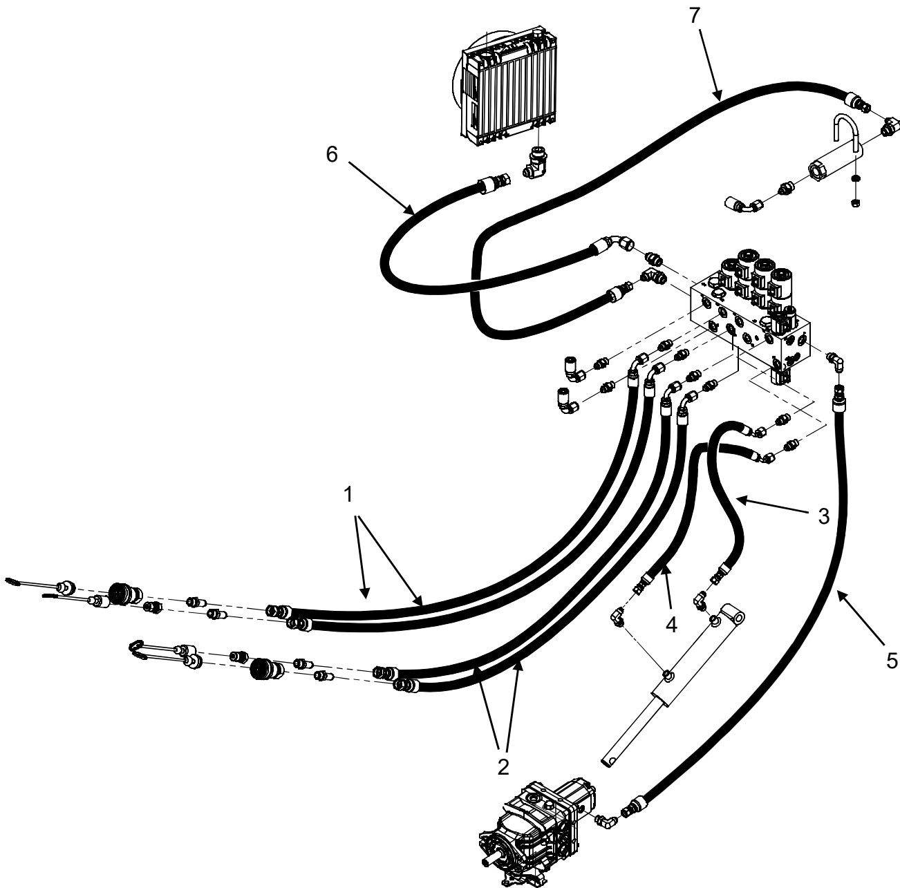
Hydraulic Hoses Group, (FC1, FC3, FC4)
